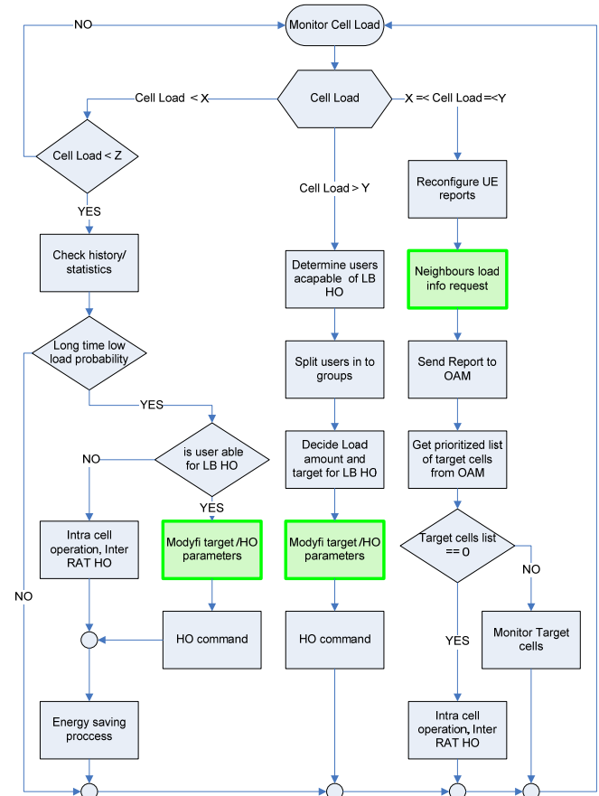
Figure 2: Load Balancing Draft Algorithm
