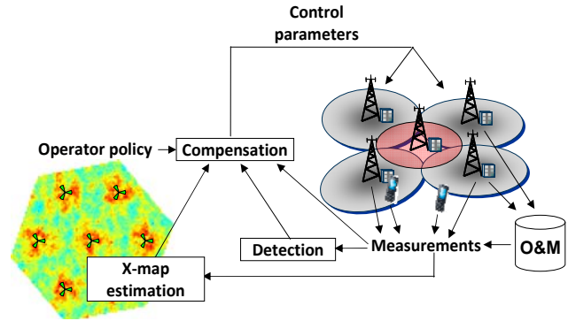
Figure 3: Cell outage management components. The center site is in outage. Red area indicates the coverage previously offered by the outage cell (Source: [5])
